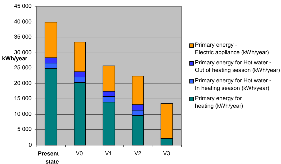
Fig. 2 Primary energy necessary to provide building operation
