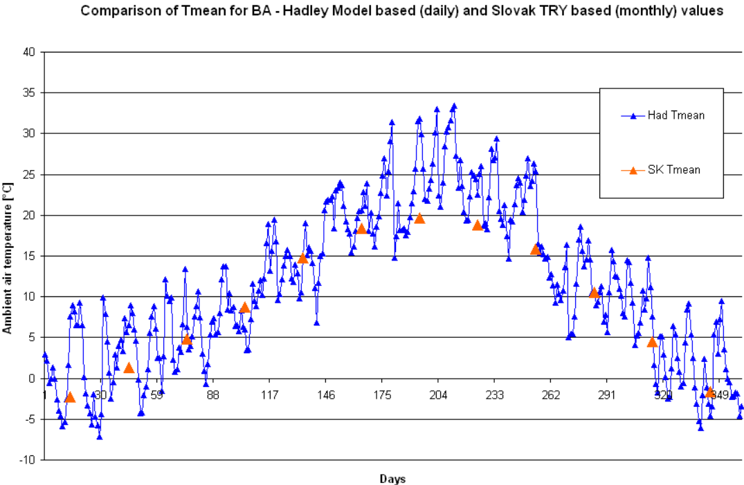
Fig. 2 Comparison of the mean ambient air temperature values of both test reference years.
