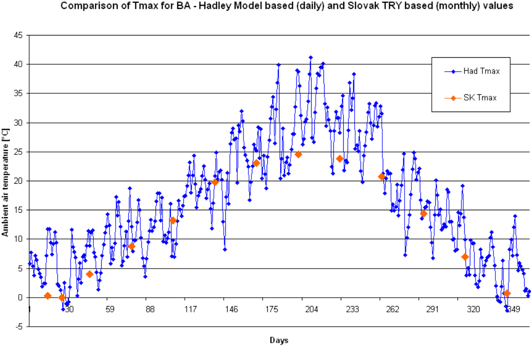
Fig. 3 Comparison of the maximum ambient air temperature values of both test reference years.
