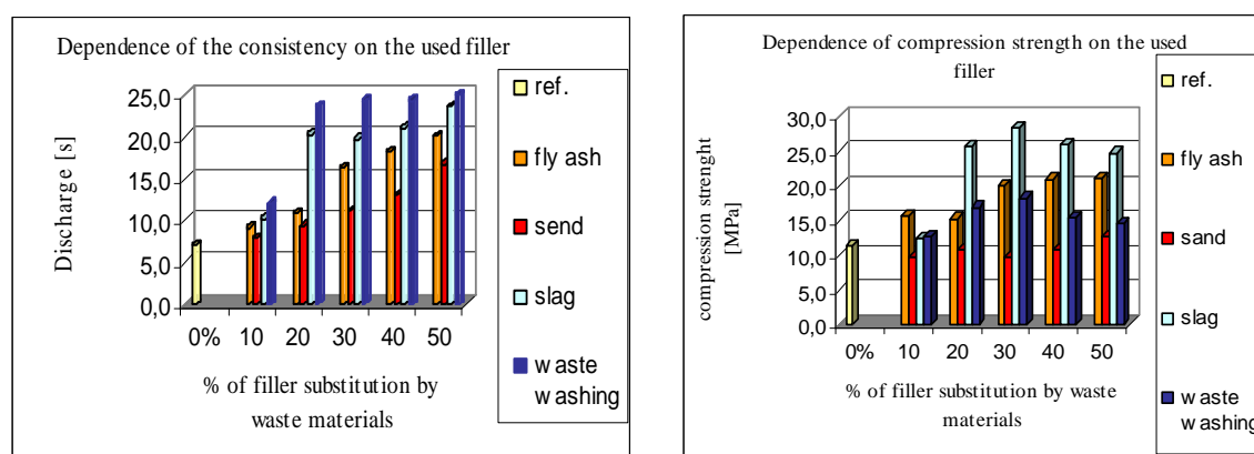
Fig. 1 a, b Dependence of the consistency and compression strength on the used filler
